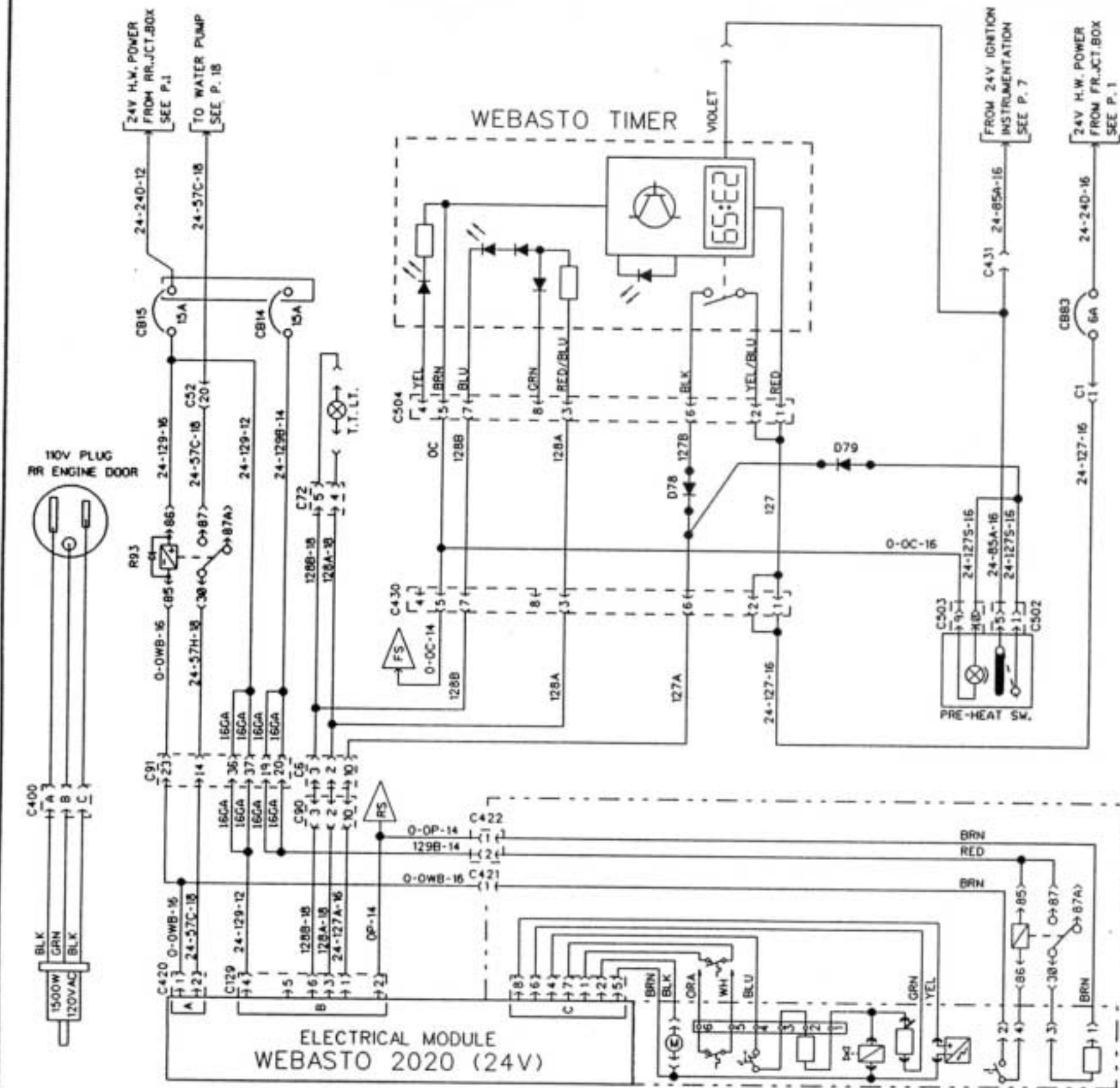
PRE-HEAT WATER HEATER (WEBASTO 2020)
